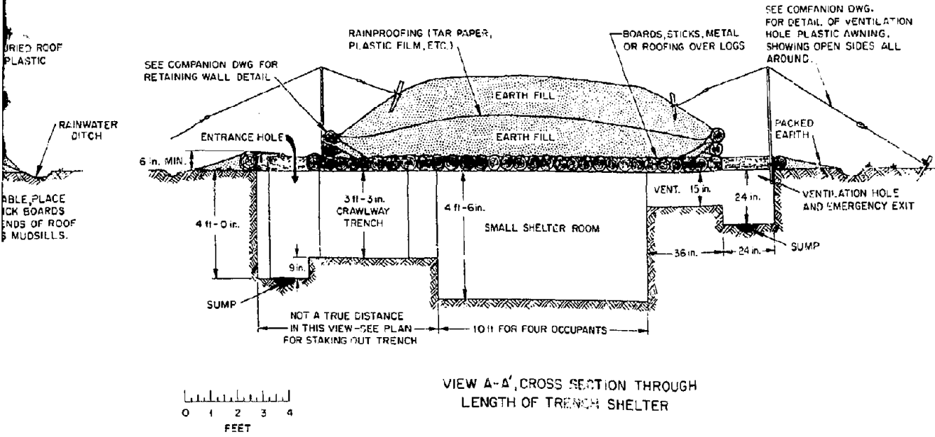
Fig. A-2.2. Log-Covered Trench Shelter, Details.
